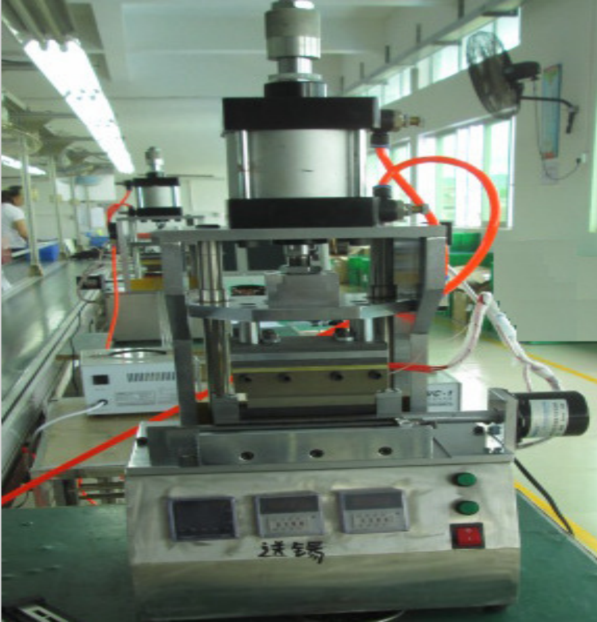
HDMI solder machine
